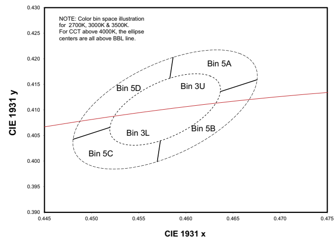
Figure 7. Color space definition for LUXEON HL2X.
