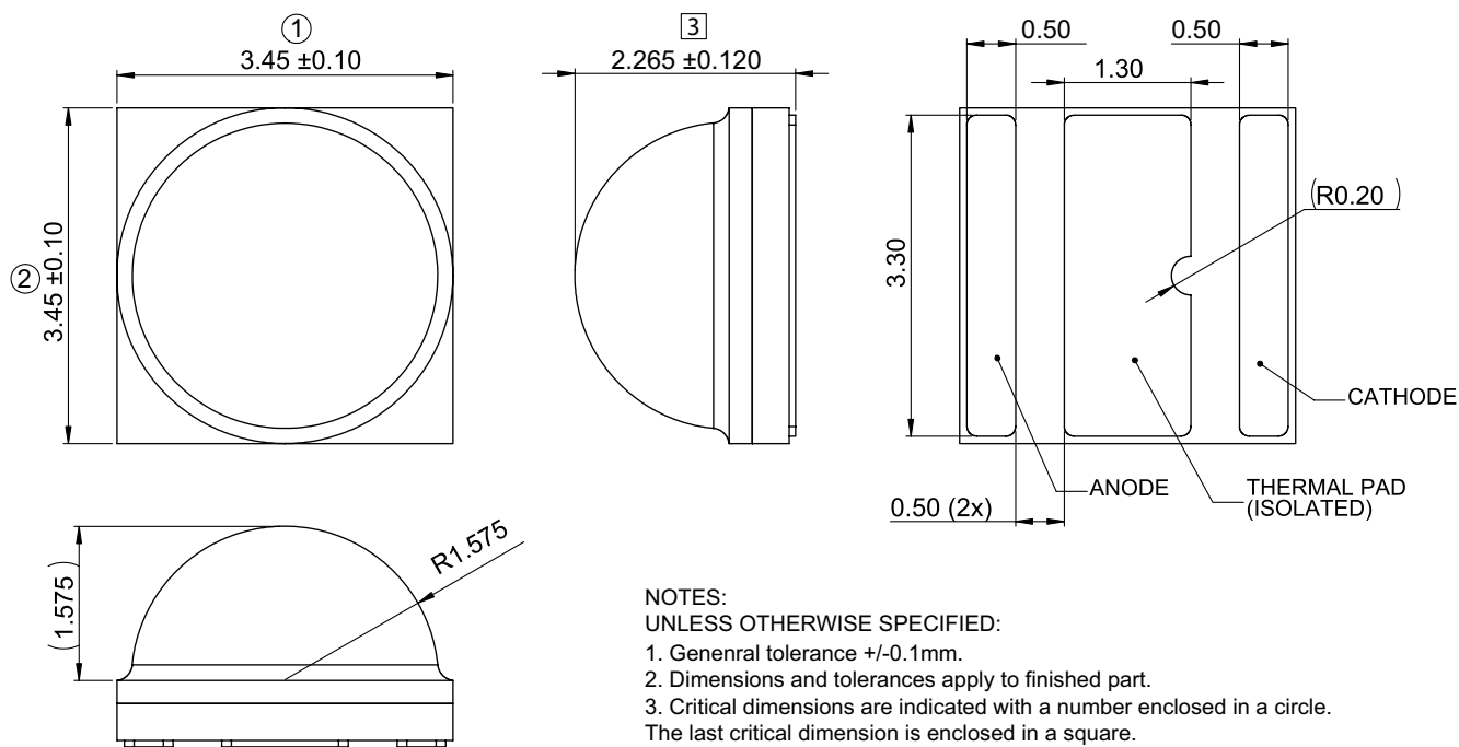
Figure 9a. Mechanical dimensions for LUXEON HL2X and LUXEON HL2X-P.
