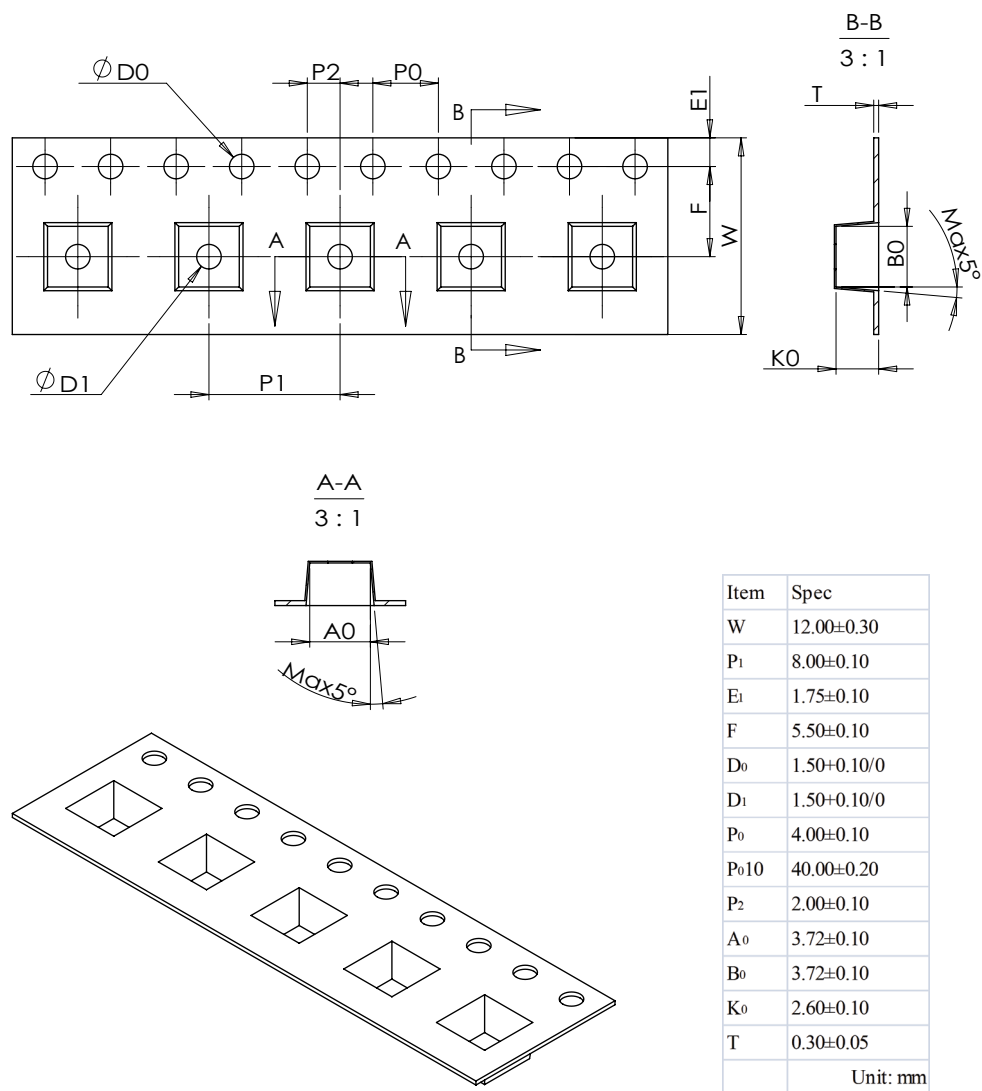
Figure 12b. Pocket tape dimensions for LUXEON HL2X-D.
